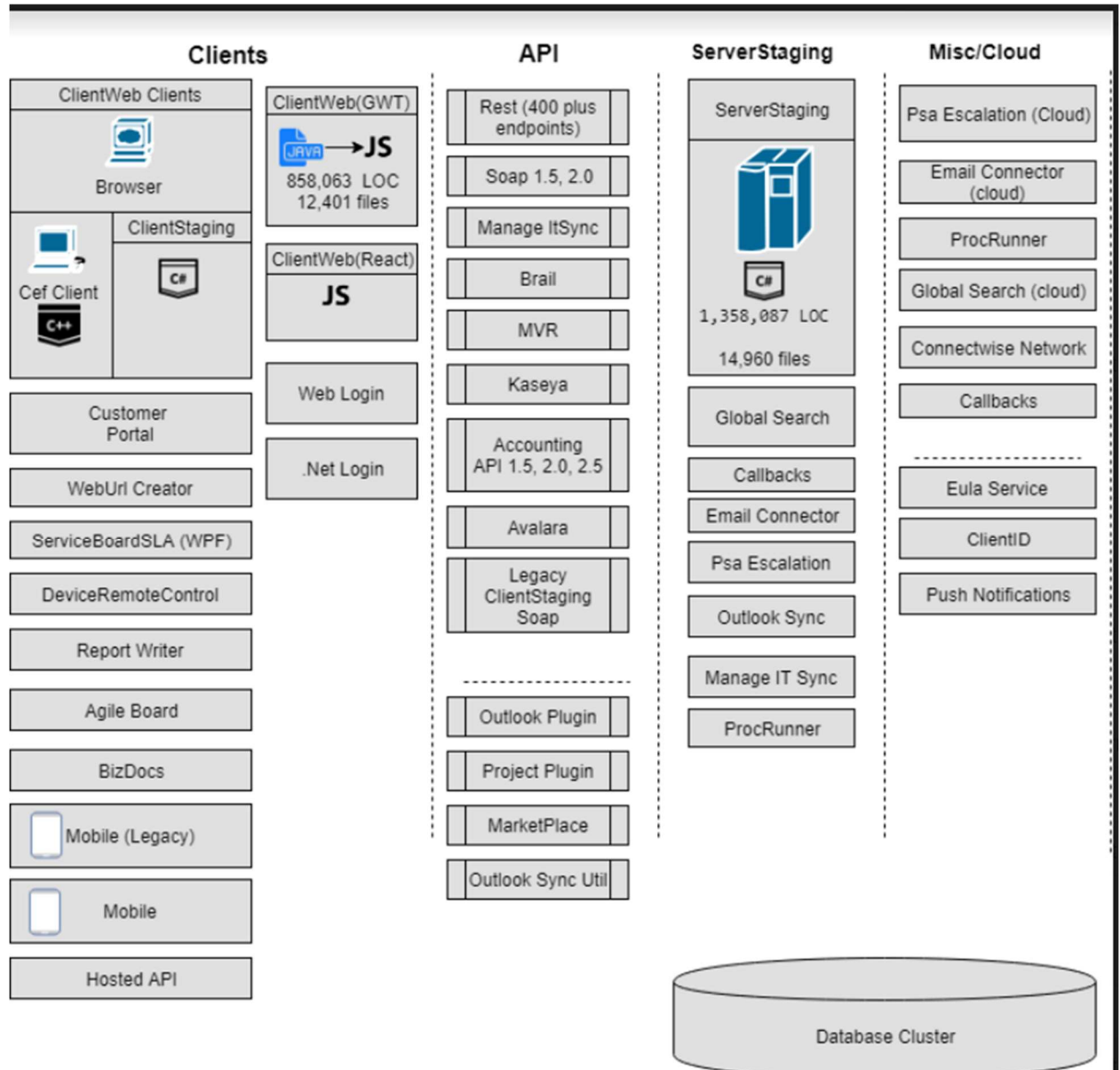
ConnectWise Manage Data Flow Diagram
